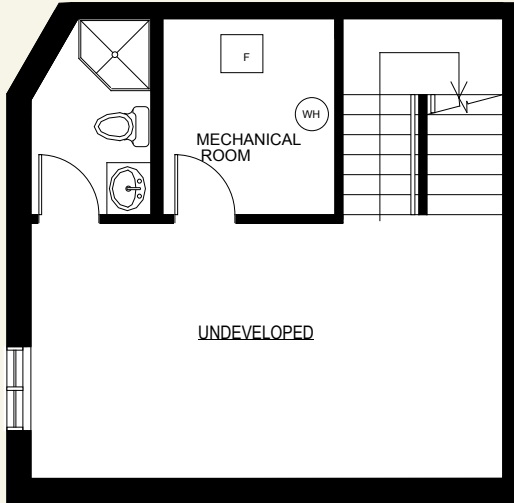
BASEMENT (427 S.F., INCL. STAIRS)
