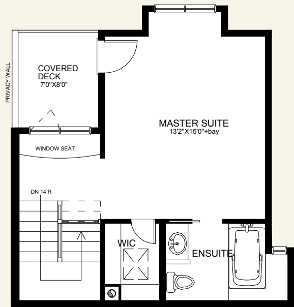
3RD FLOOR (437 S.F., INCL. STAIRS)
